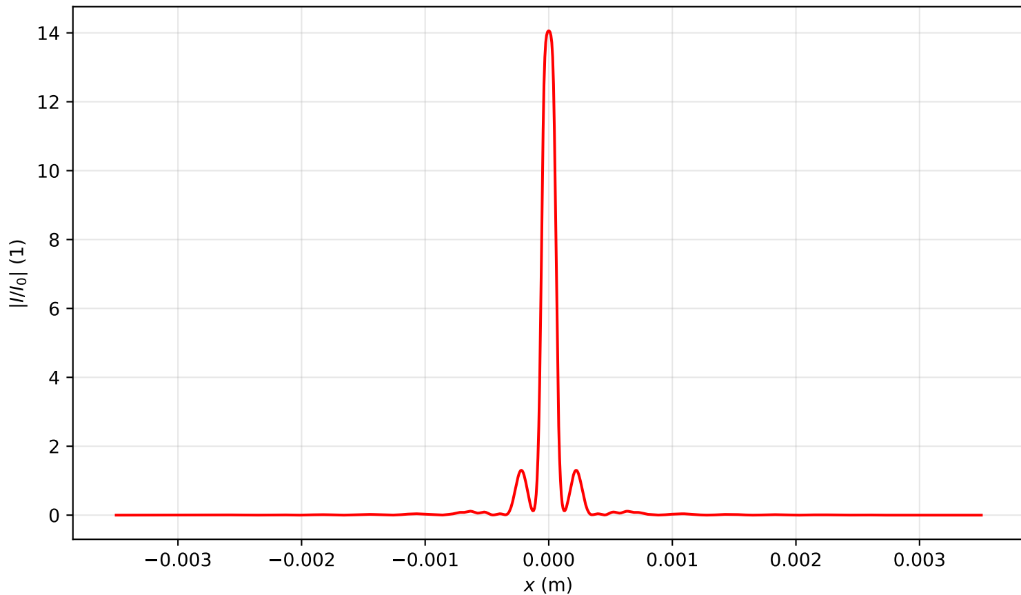
Intensity profile I(x, y = 0, z = 0.318)/I_0 , P_{in}=5.0P_{cr} , artificial time
